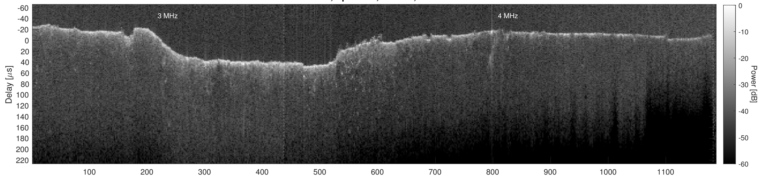
Orbit 8359, Cluttergram
