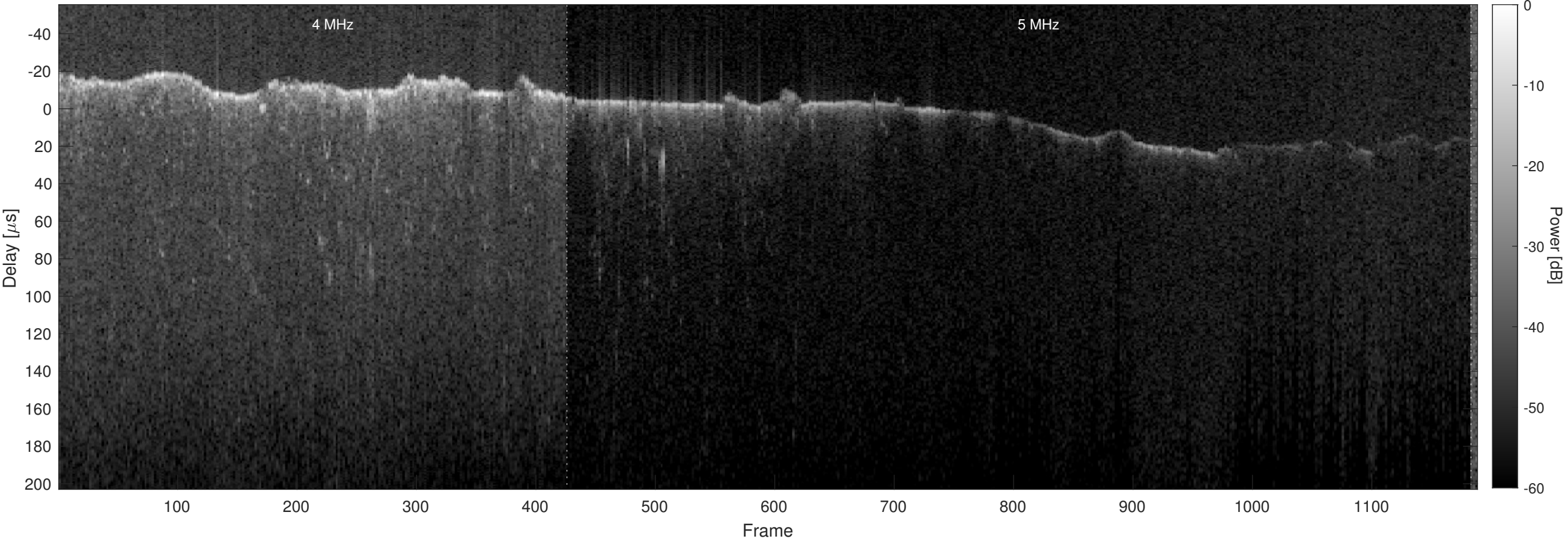
Orbit 8361, Optimized, Window, Channel 2
