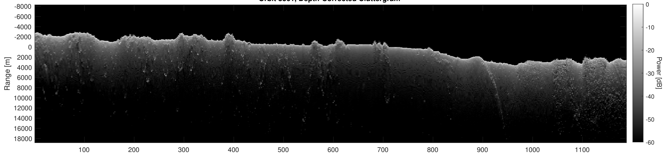
Orbit 8361, Depth-Corrected Cluttergram
