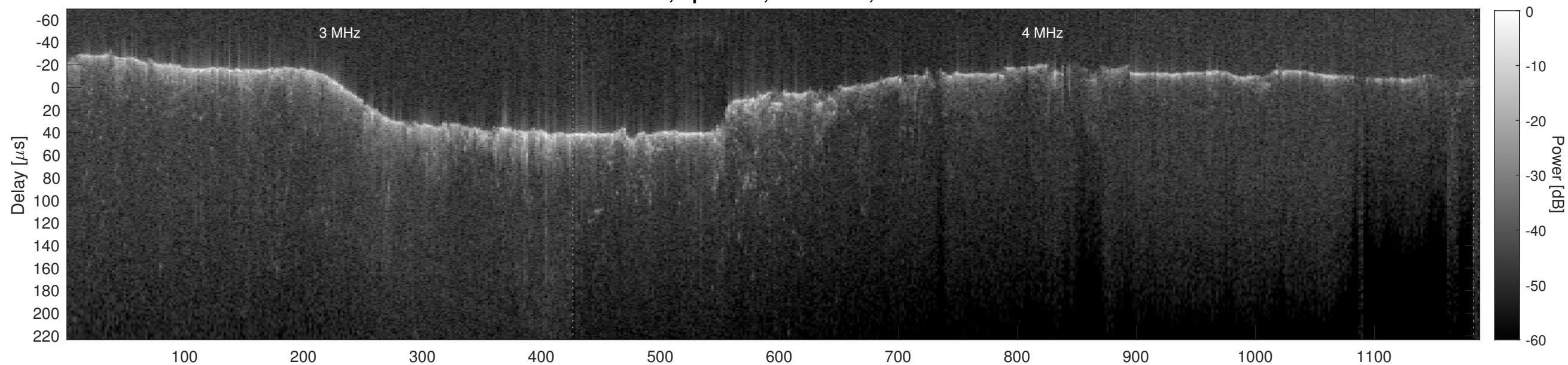
Orbit 8366, Cluttergram
