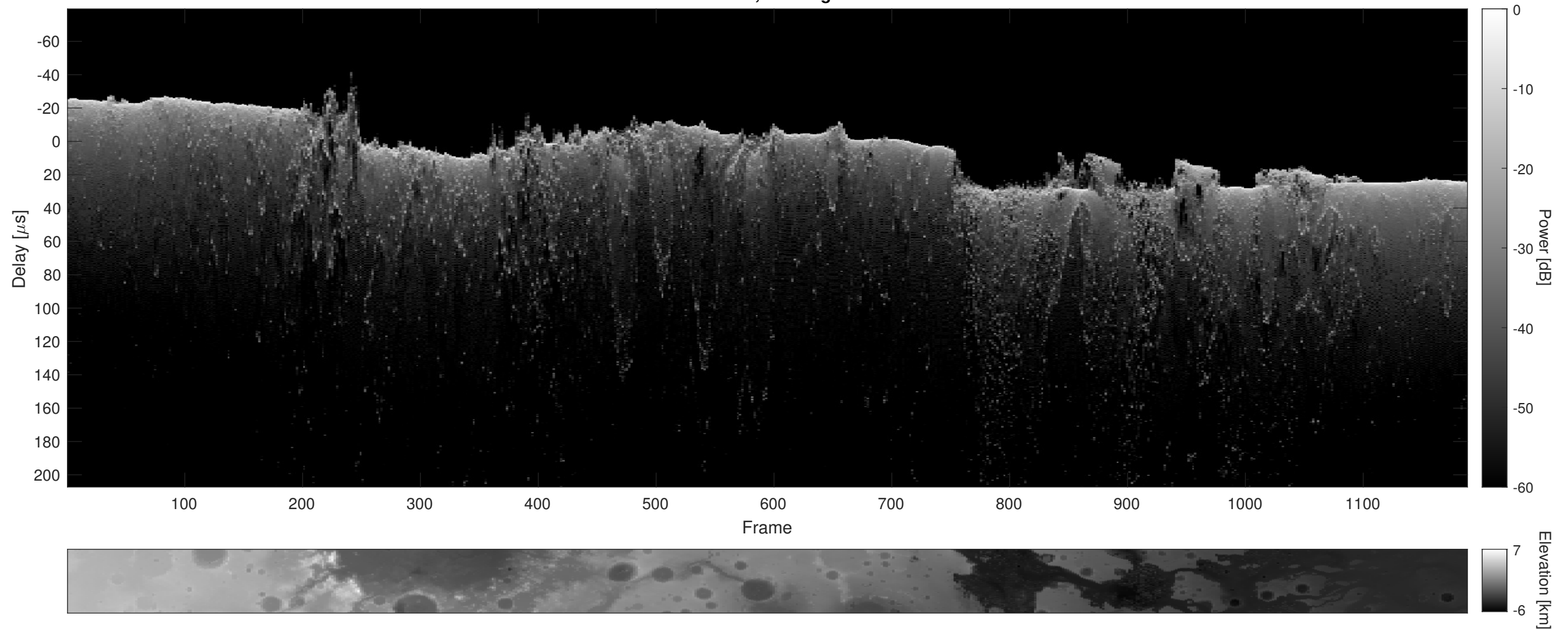
Orbit 8367, Cluttergram
