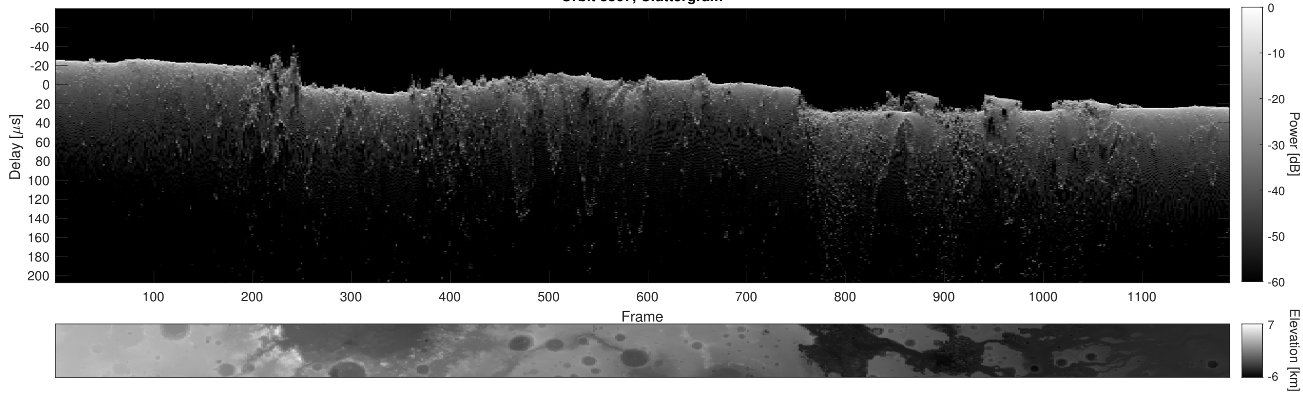
Orbit 8367, Cluttergram
