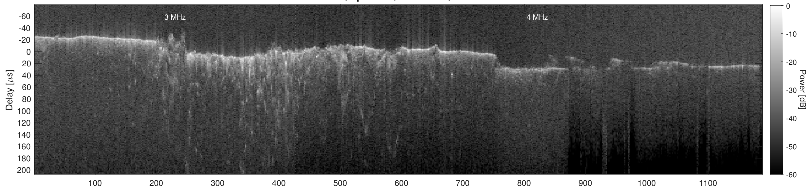
Orbit 8367, Cluttergram
