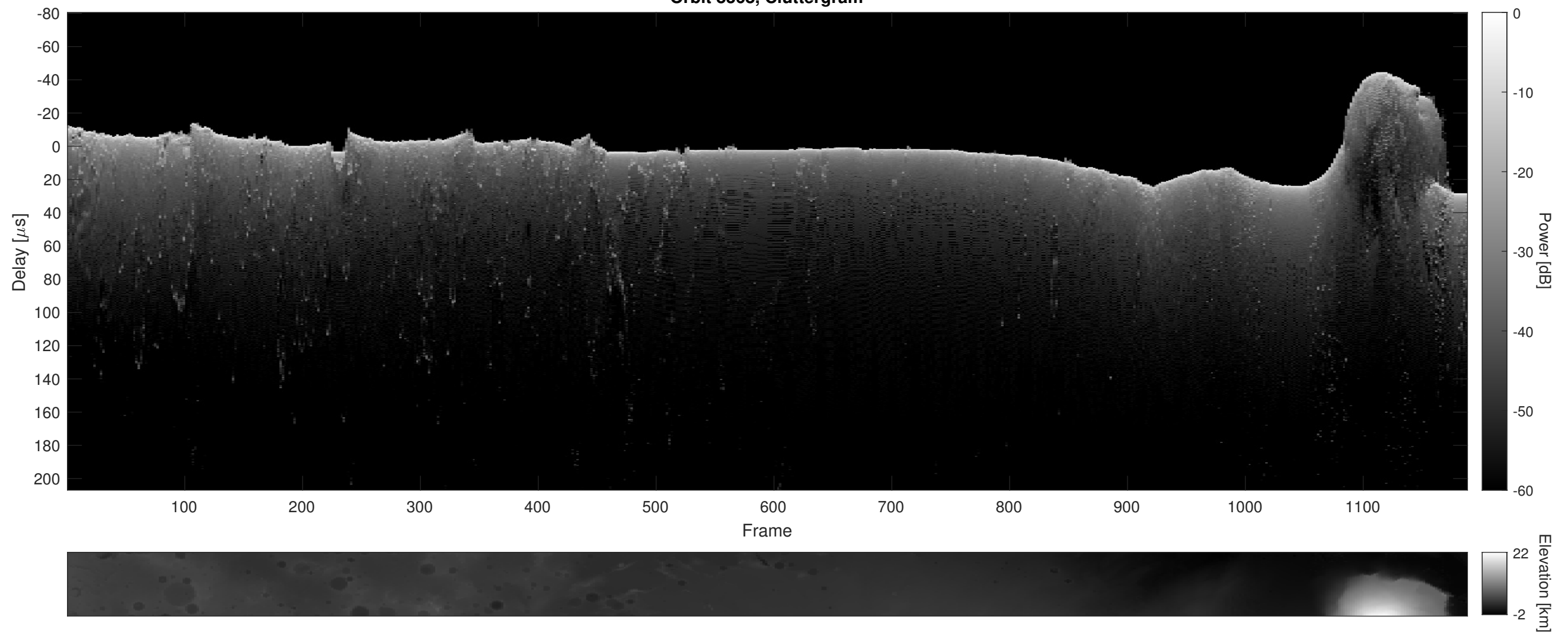
Orbit 8368, Cluttergram
