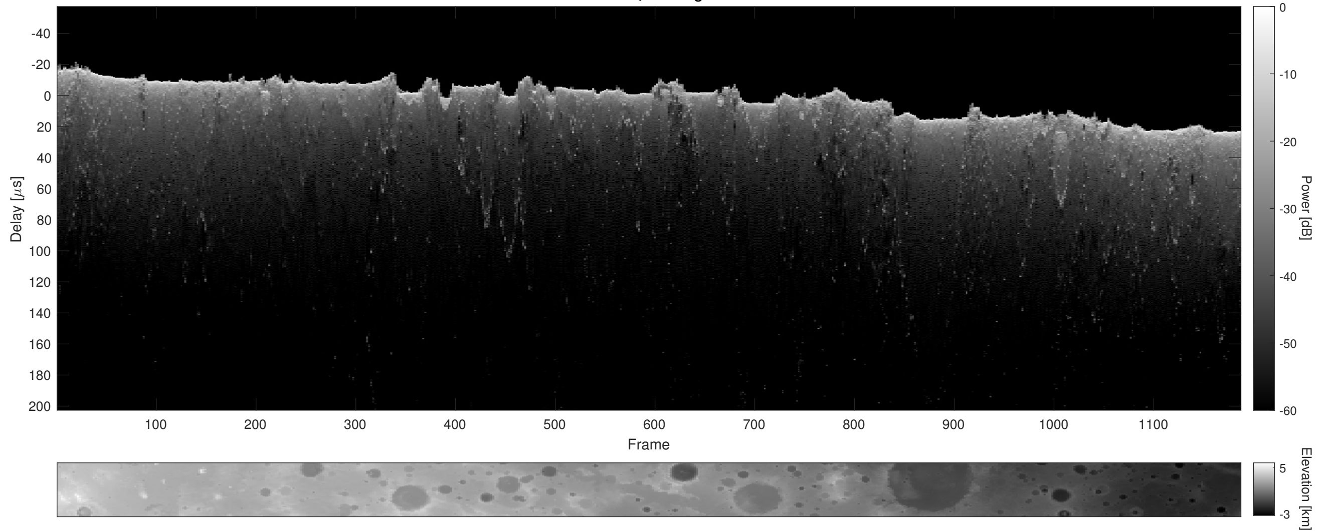
Orbit 8370, Cluttergram
