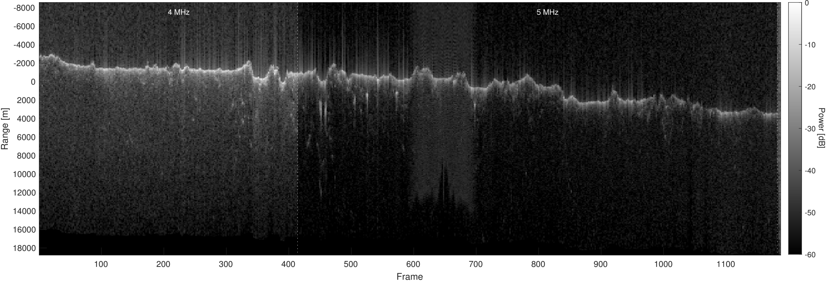
Orbit 8370, Optimized, No Window, Depth-Corrected, Channel 2
