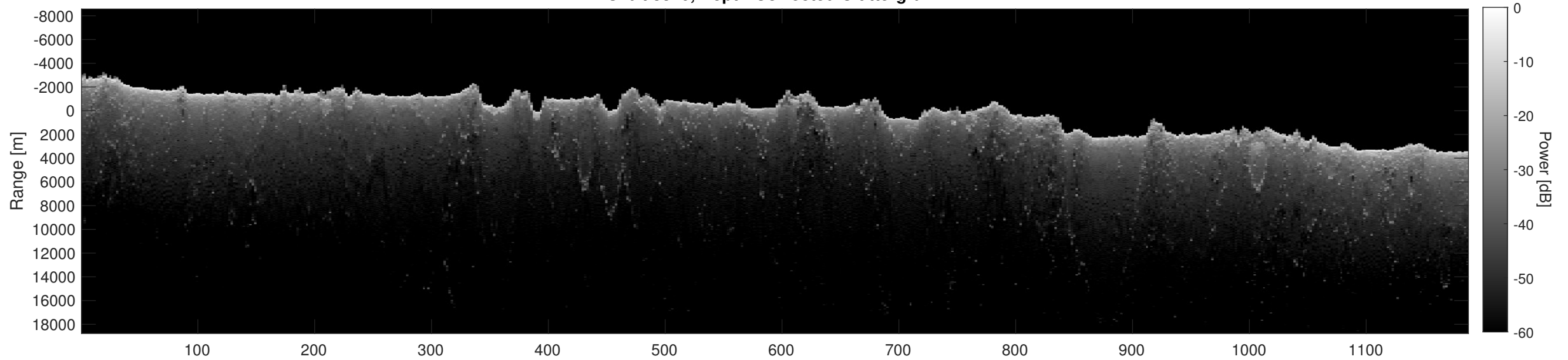
Orbit 8370, Depth-Corrected Cluttergram
