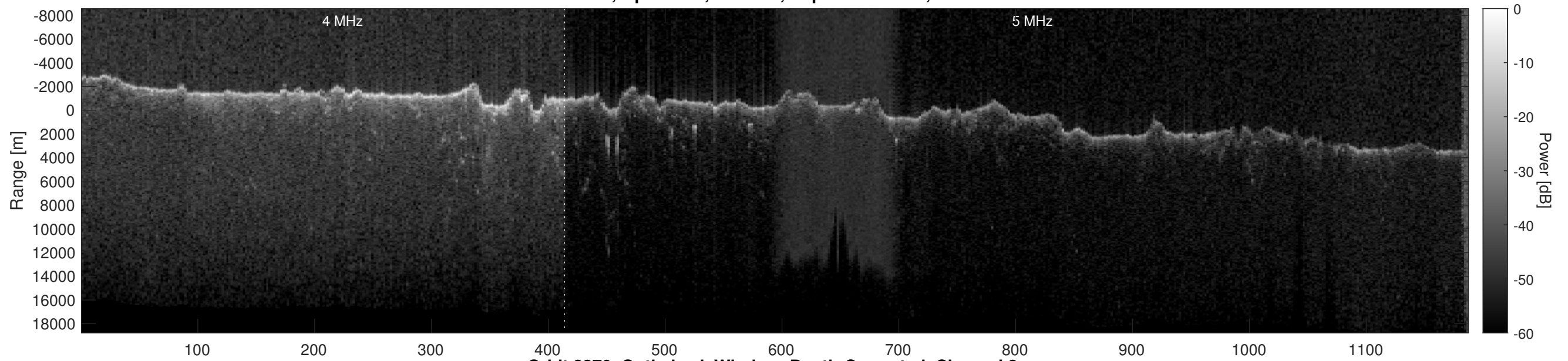
Orbit 8370, Optimized, Window, Depth-Corrected, Channel 2
