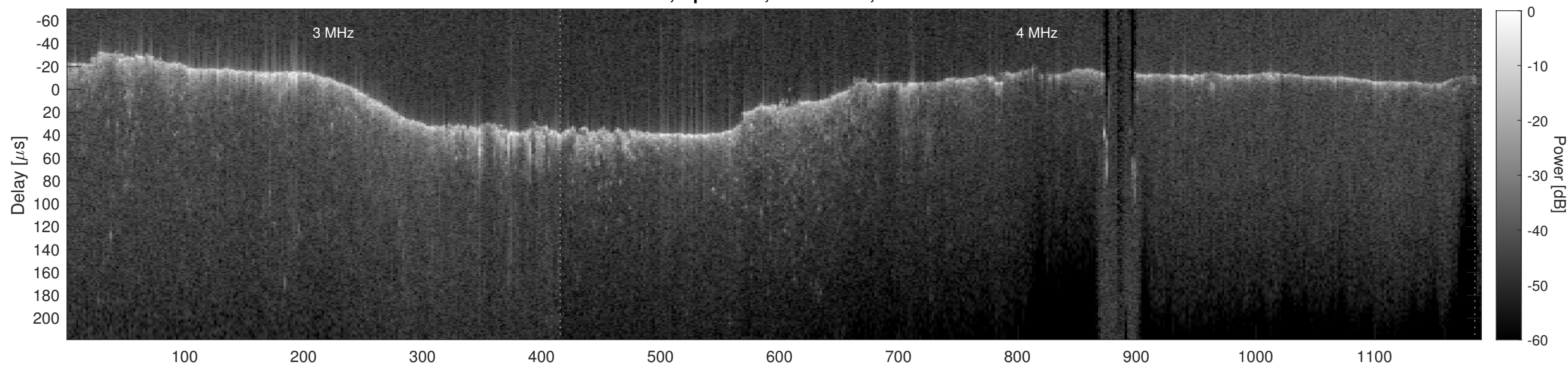
Orbit 8373, Cluttergram
