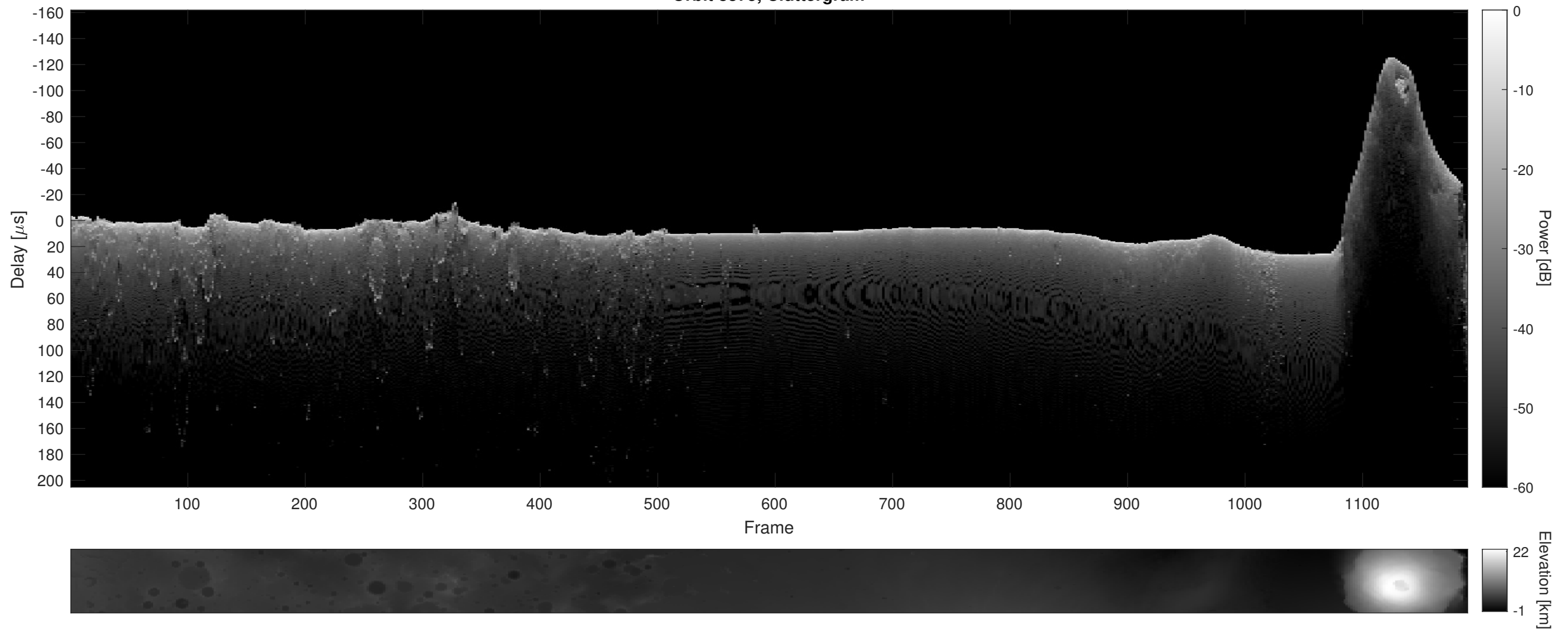
Orbit 8375, Cluttergram
