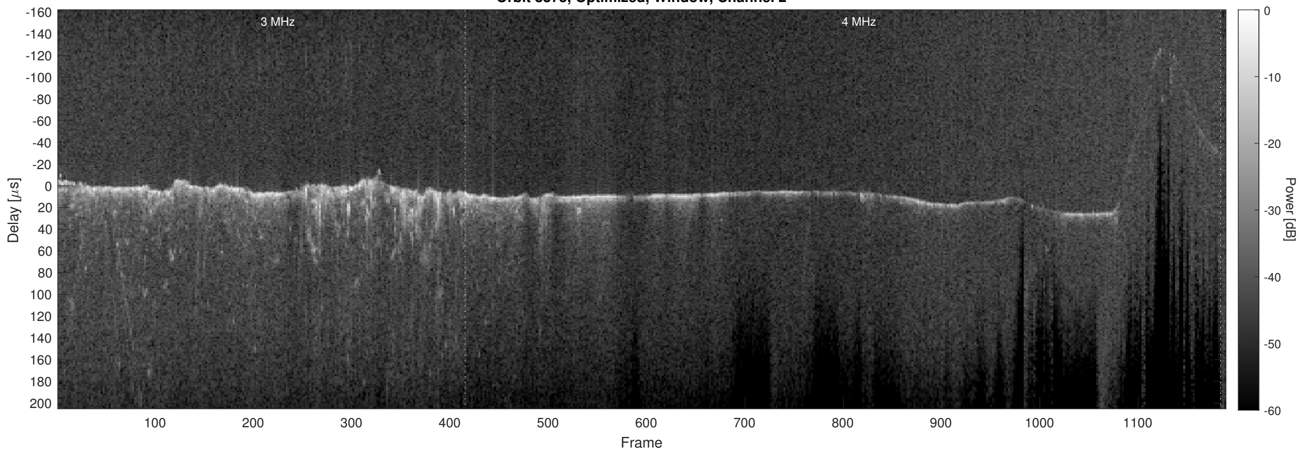
Orbit 8375, Optimized, Window, Channel 2
