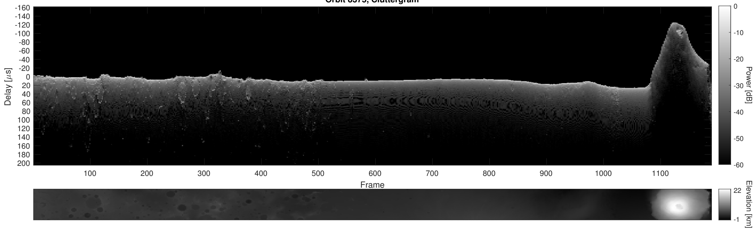
Orbit 8375, Cluttergram
