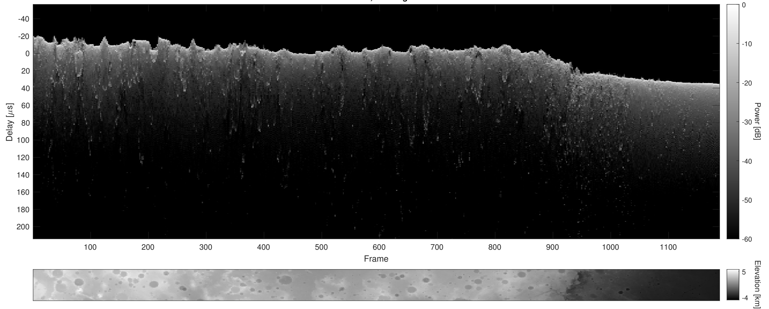
Orbit 8376, Cluttergram
