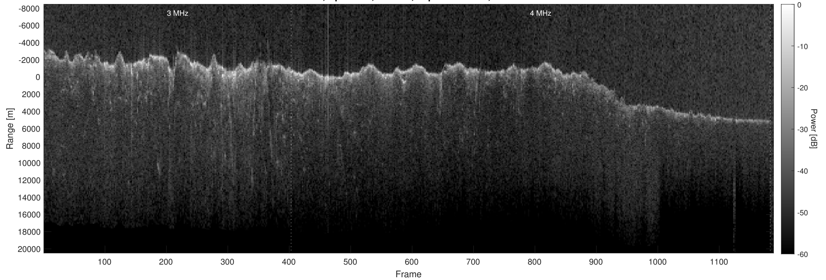
Orbit 8376, Optimized, Window, Depth-Corrected, Channel 2
