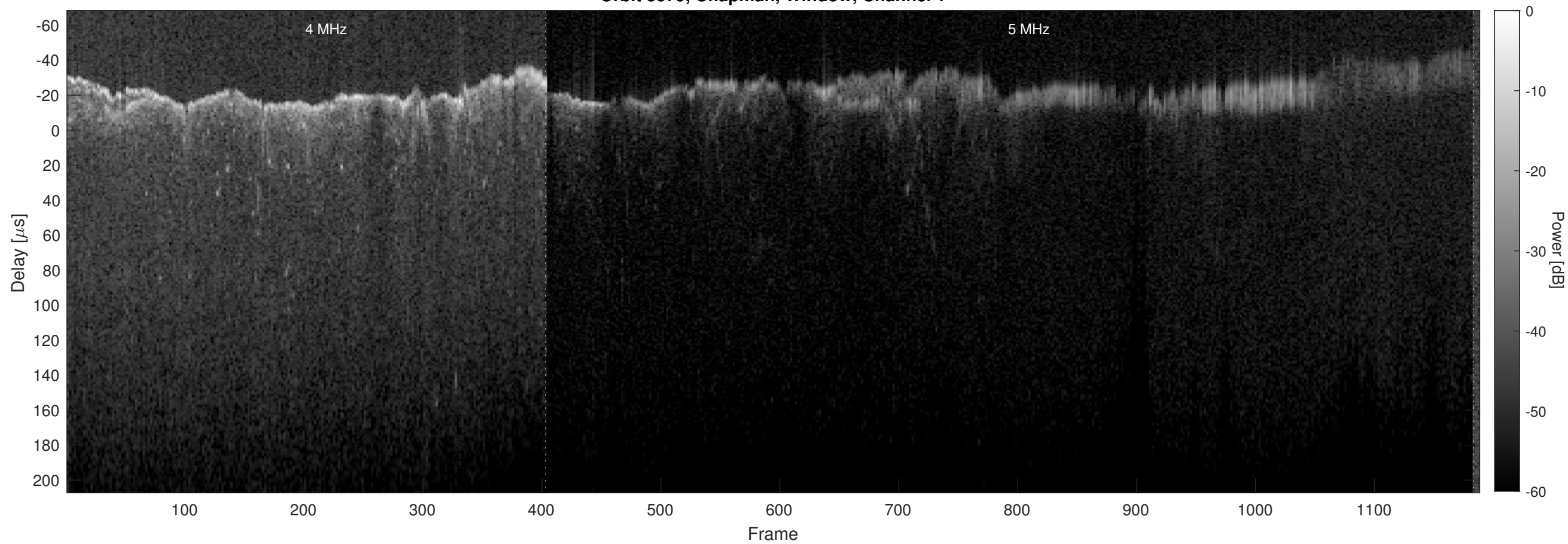
Orbit 8379, Chapman, Window, Channel 2
