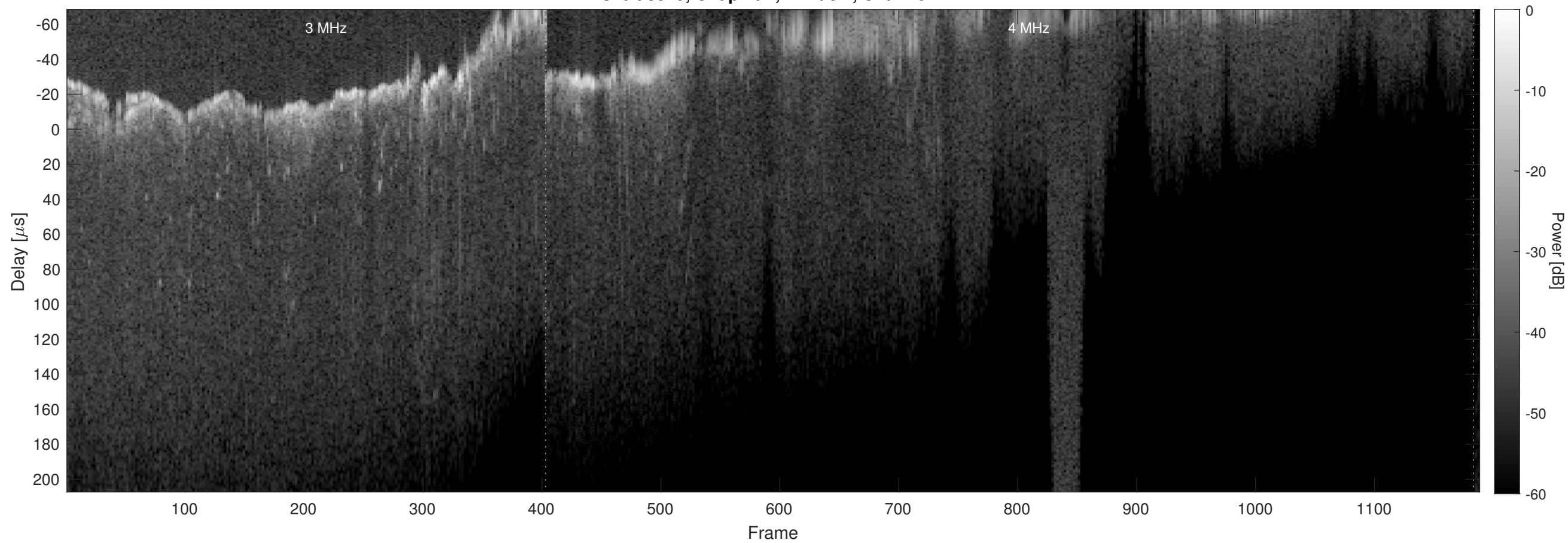
Orbit 8379, Chapman, Window, Channel 2
