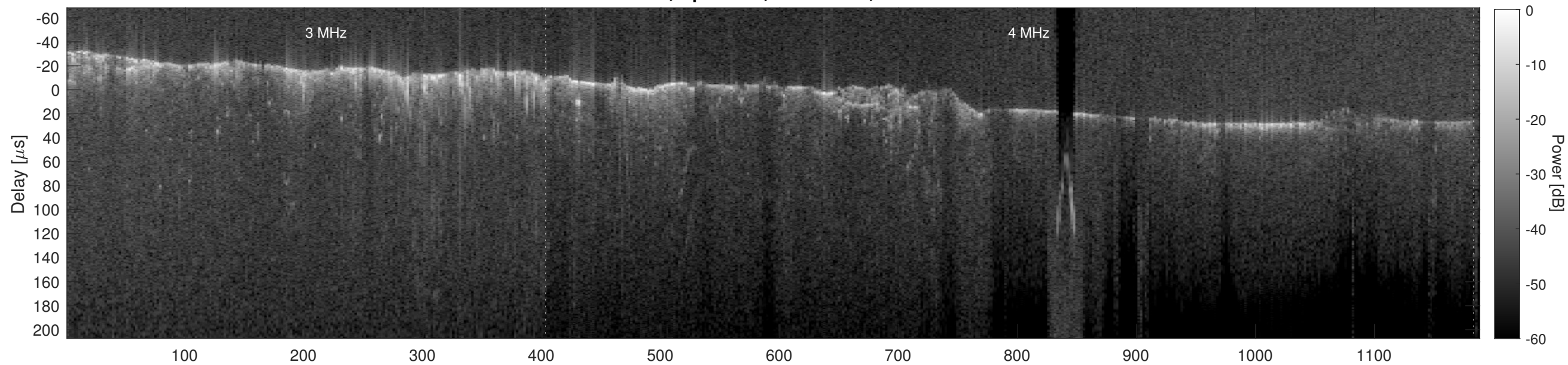
Orbit 8379, Cluttergram
