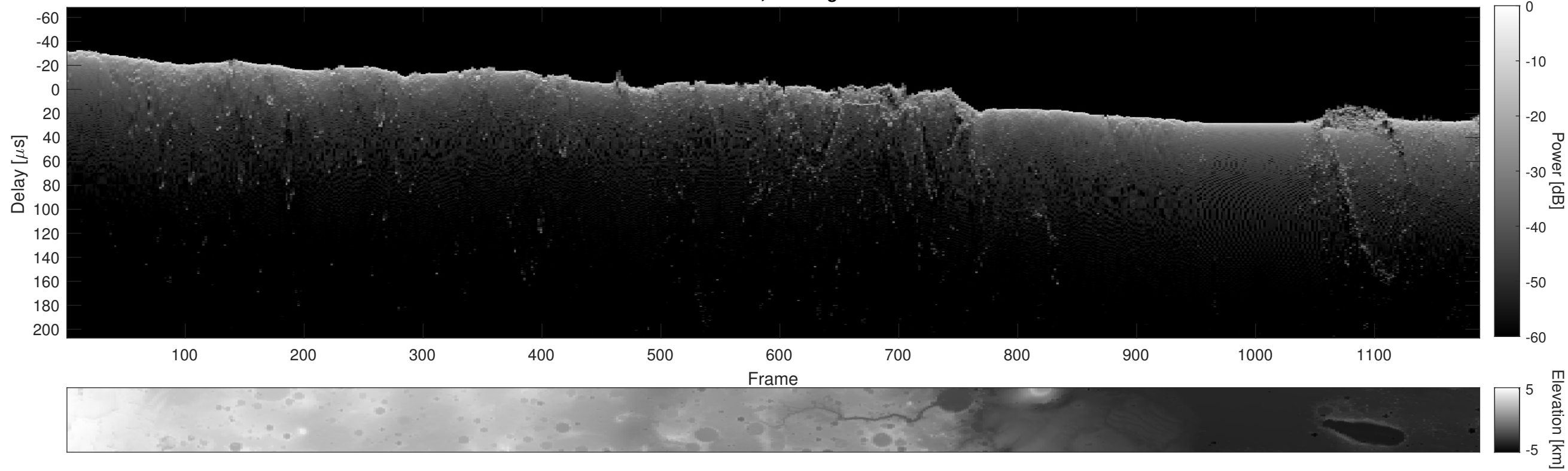
Orbit 8379, Cluttergram
