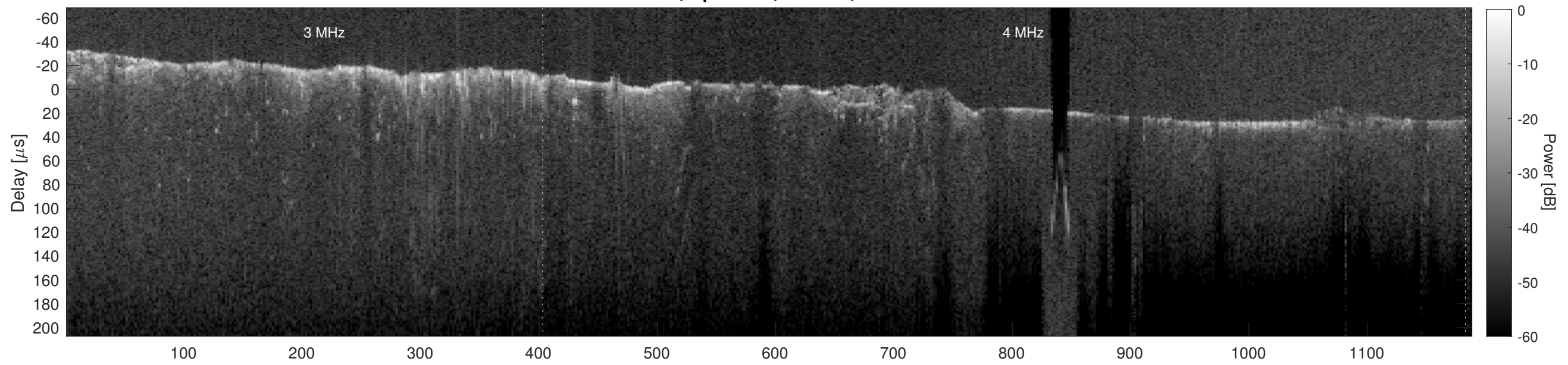
Orbit 8379, Cluttergram
