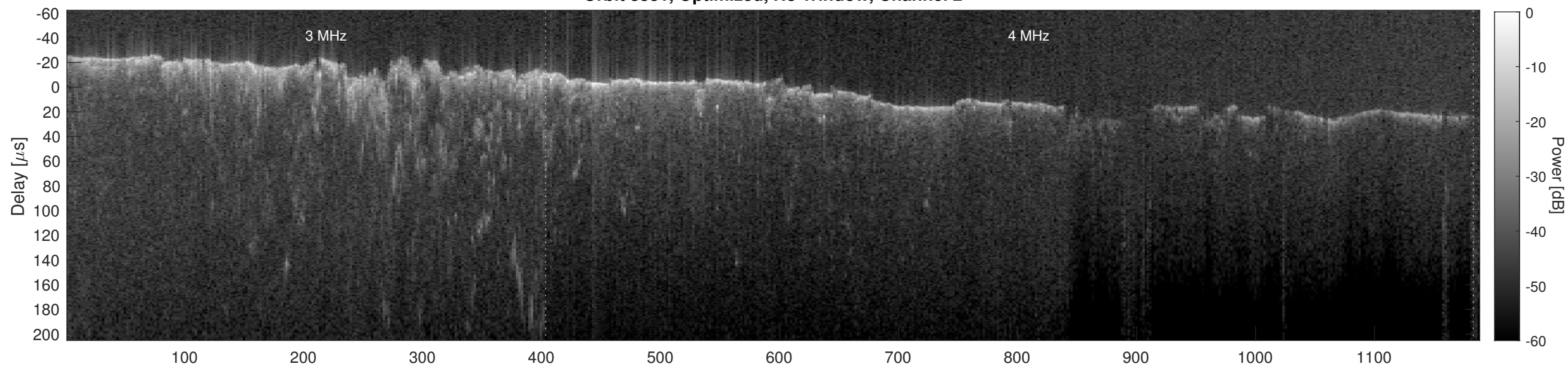
Orbit 8381, Cluttergram
