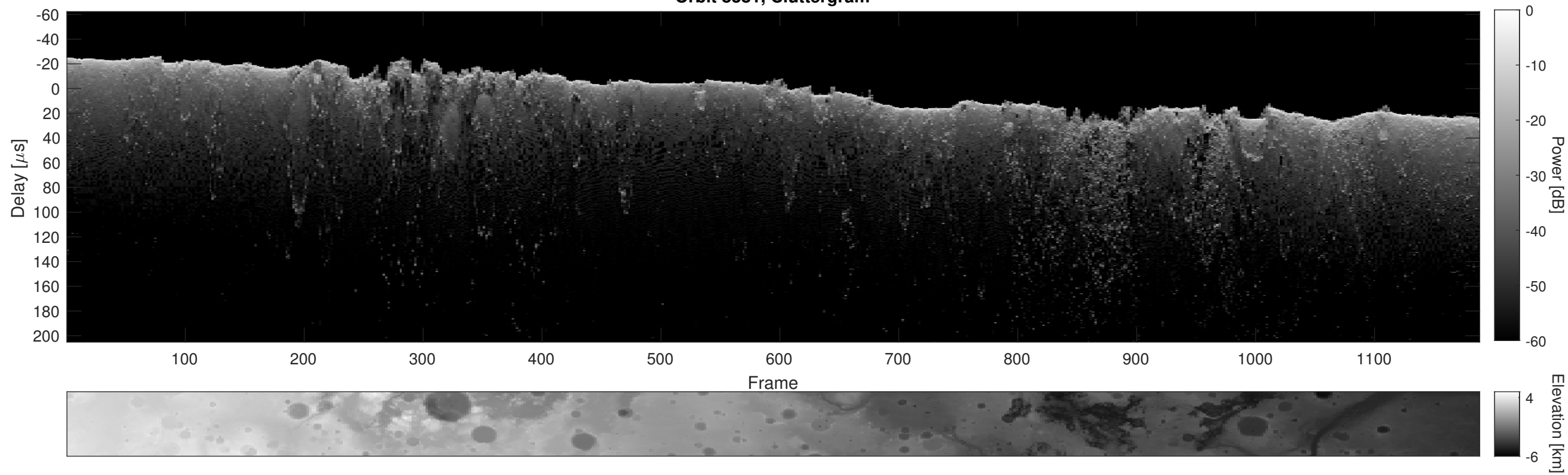
Orbit 8381, Cluttergram
