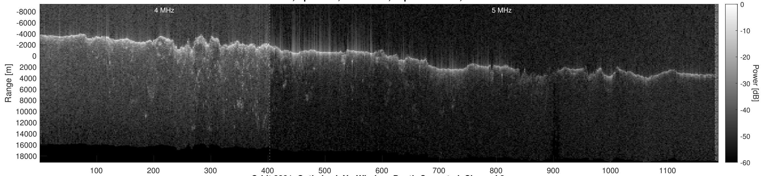
Orbit 8381, Optimized, No Window, Depth-Corrected, Channel 2
