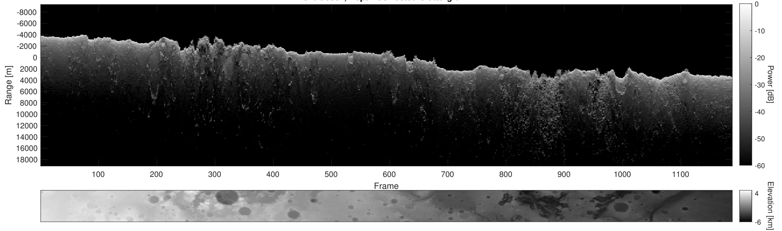
Orbit 8381, Depth-Corrected Cluttergram
