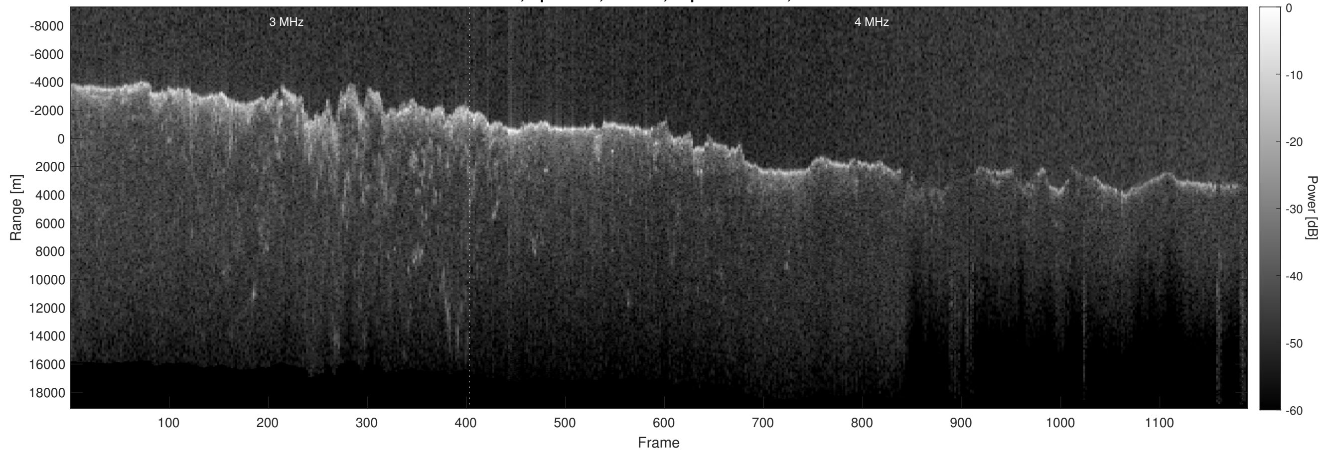
Orbit 8381, Optimized, Window, Depth-Corrected, Channel 2
