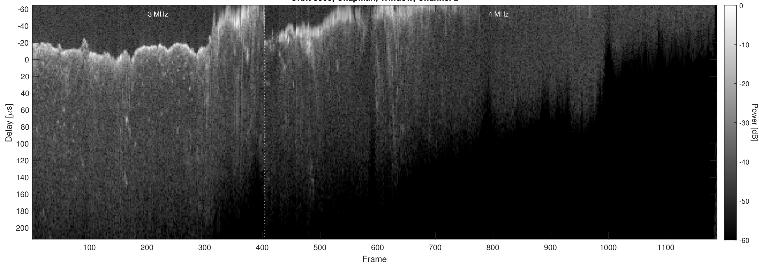
Orbit 8383, Chapman, Window, Channel 2
