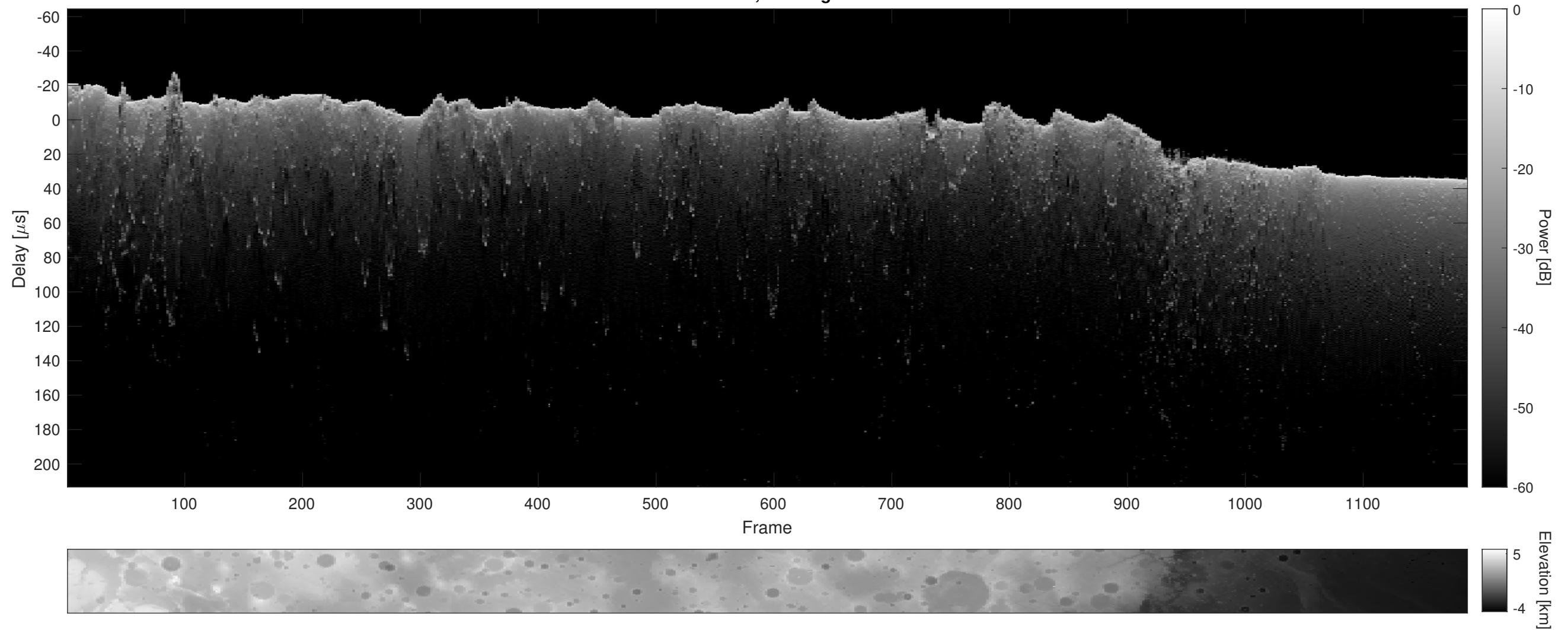
Orbit 8383, Cluttergram
