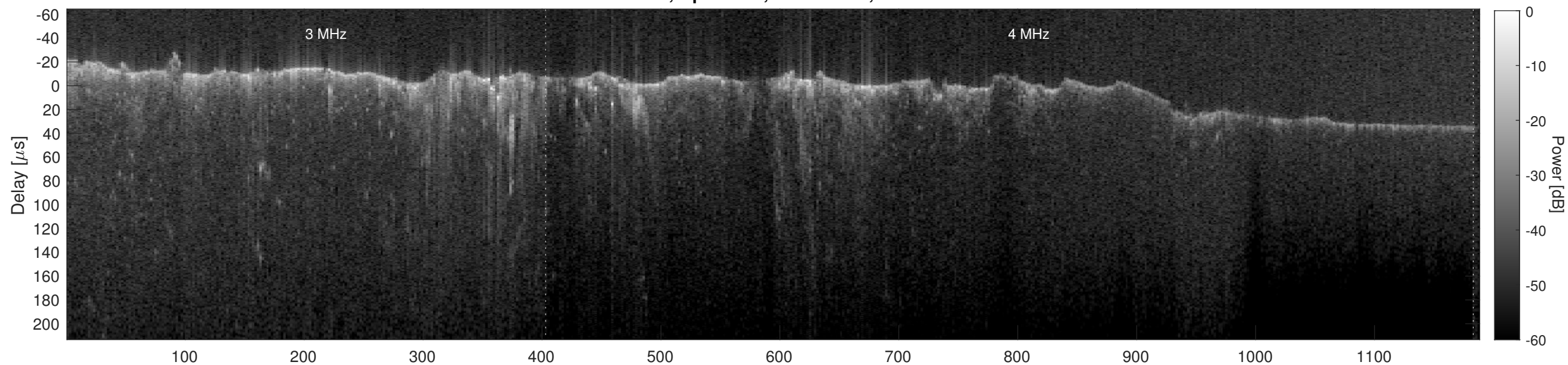
Orbit 8383, Cluttergram
