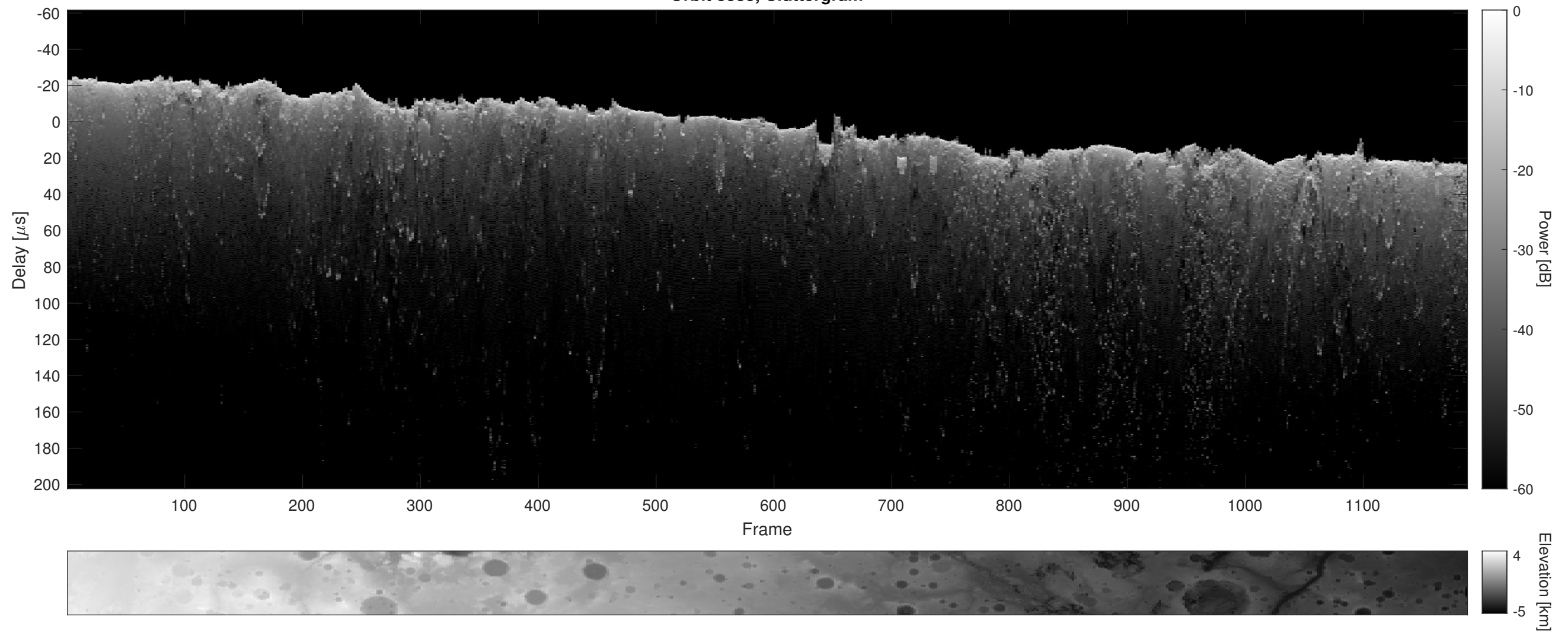
Orbit 8388, Cluttergram
