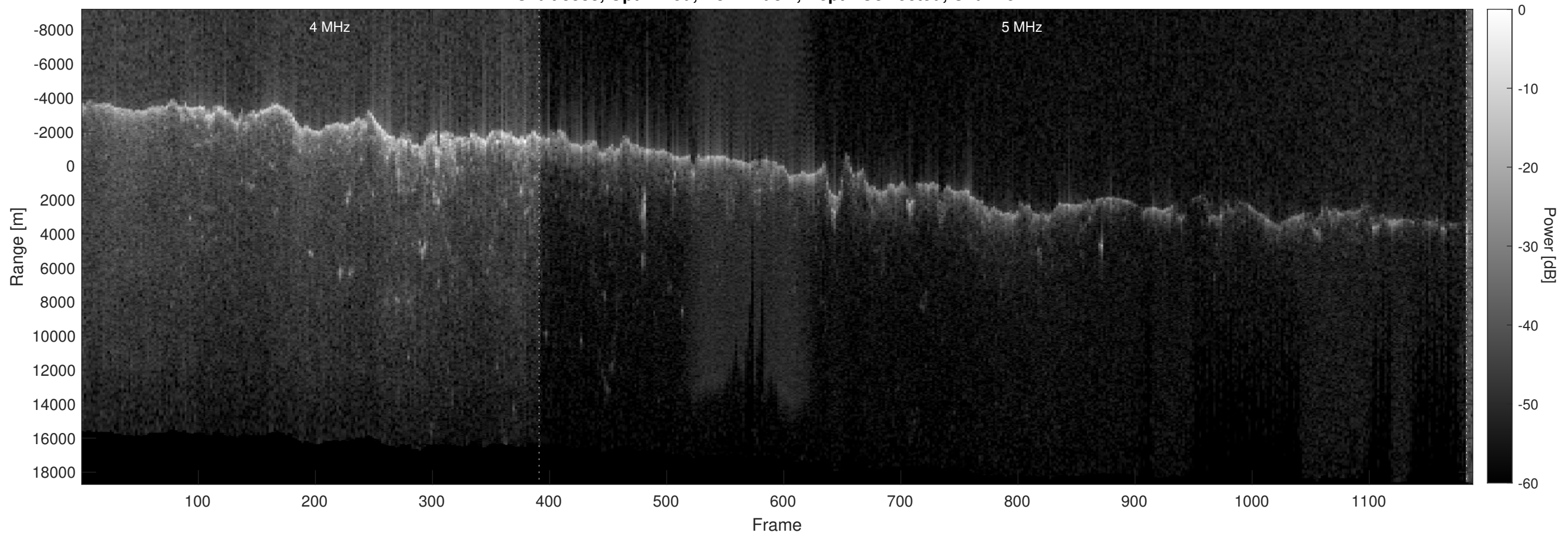
Orbit 8388, Optimized, No Window, Depth-Corrected, Channel 2
