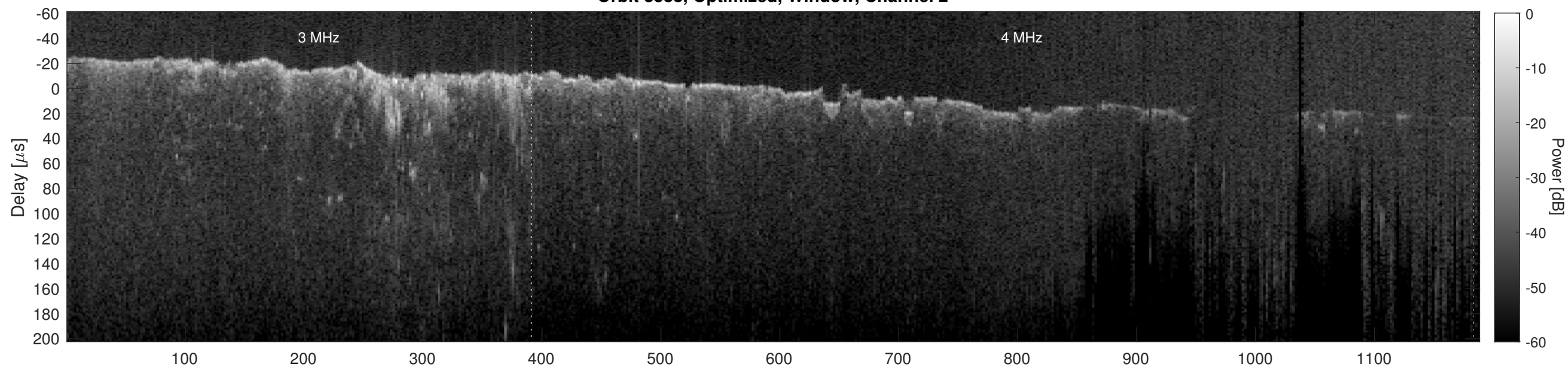
Orbit 8388, Cluttergram
