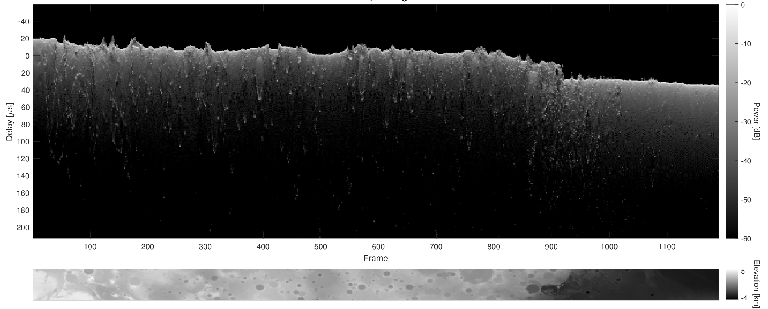
Orbit 8390, Cluttergram
