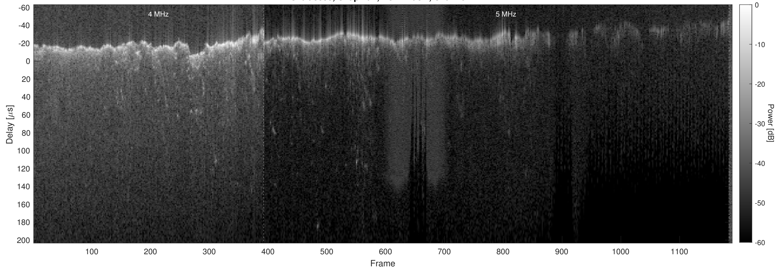
Orbit 8395, Chapman, No Window, Channel 2
