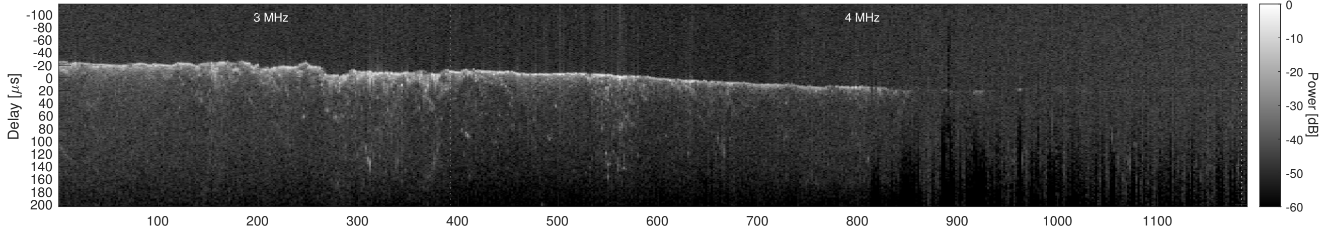
Orbit 8395, Cluttergram
