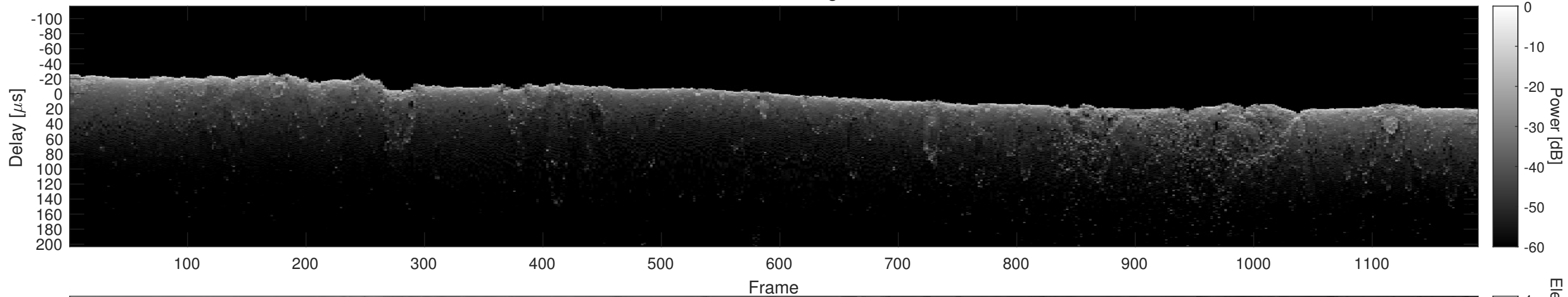
Orbit 8395, Cluttergram
