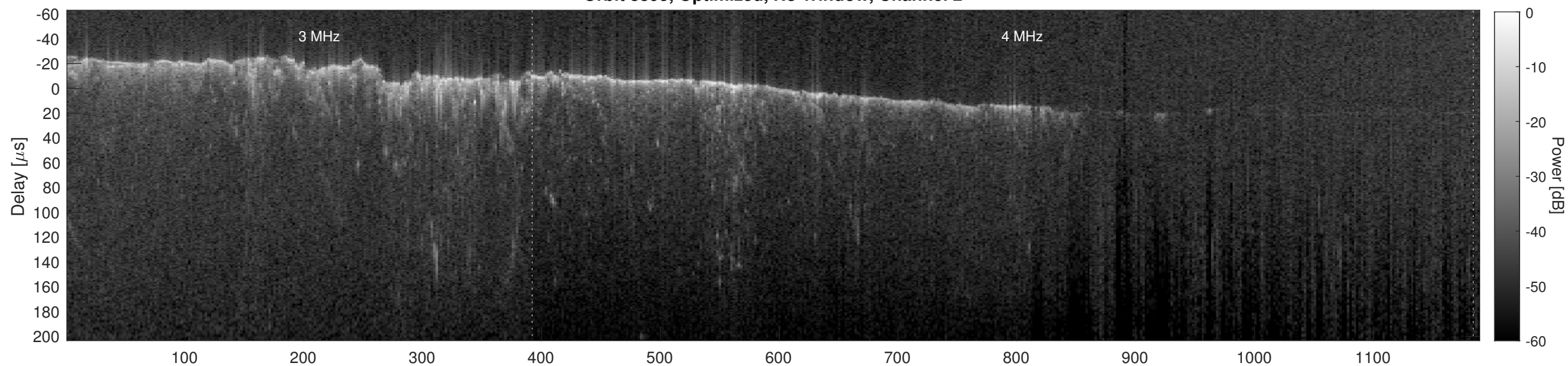
Orbit 8395, Cluttergram
