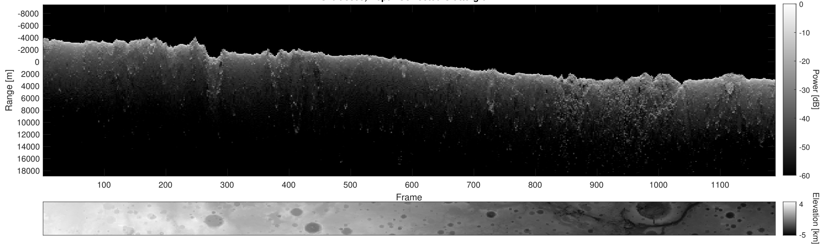
Orbit 8395, Depth-Corrected Cluttergram
