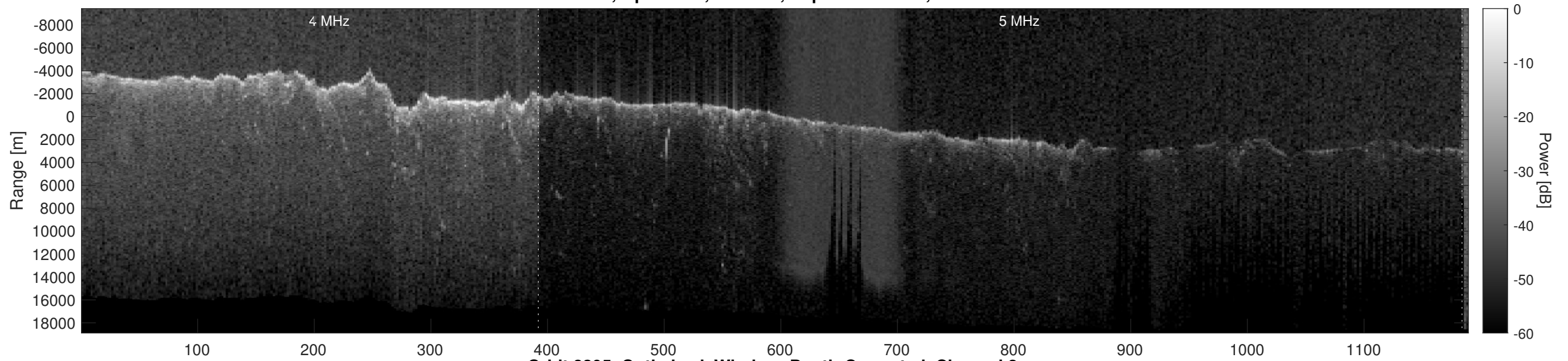
Orbit 8395, Optimized, Window, Depth-Corrected, Channel 2
