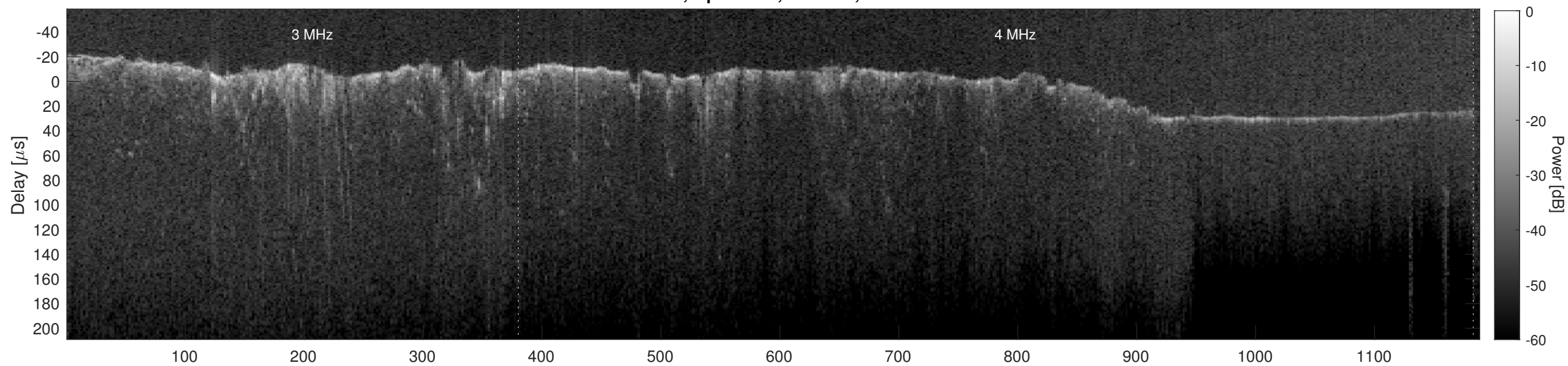
Orbit 8397, Cluttergram
