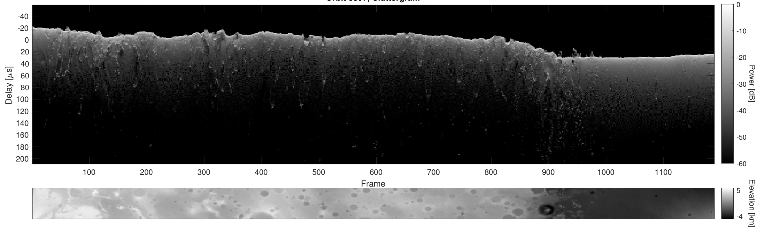
Orbit 8397, Cluttergram
