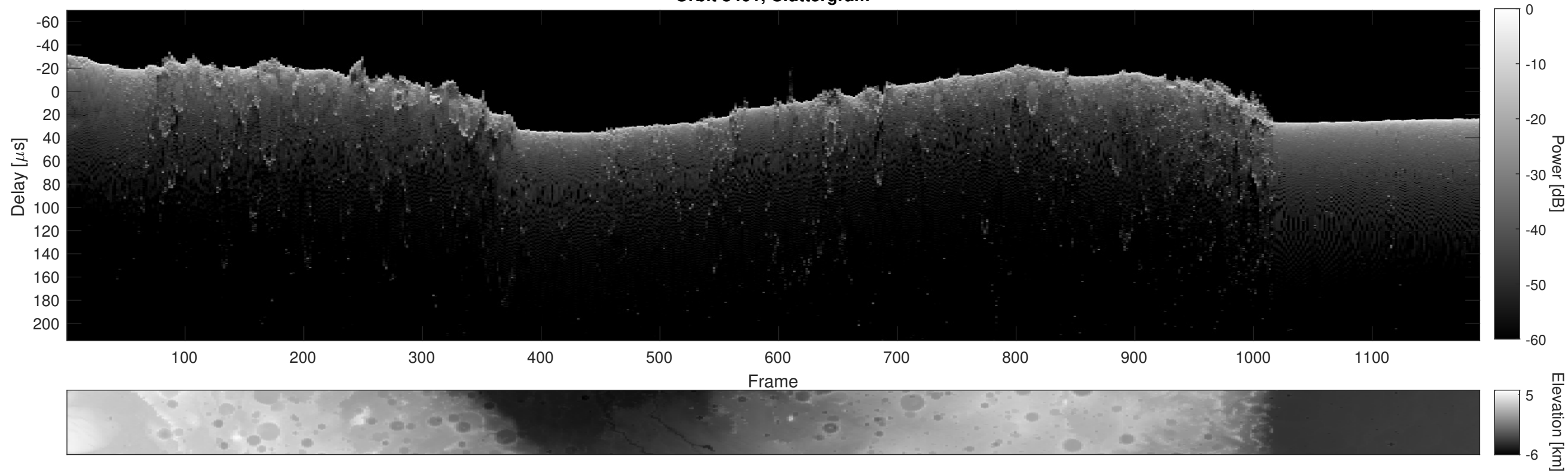
Orbit 8401, Cluttergram
