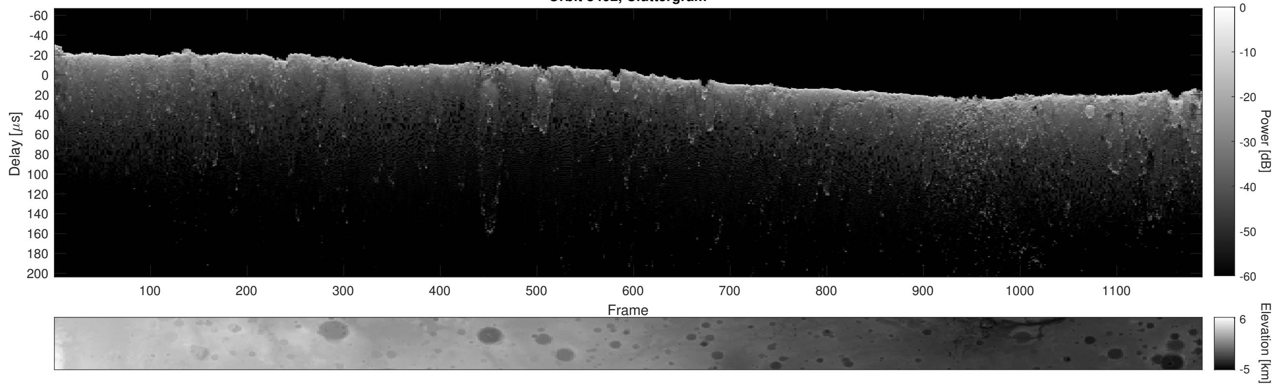
Orbit 8402, Cluttergram
