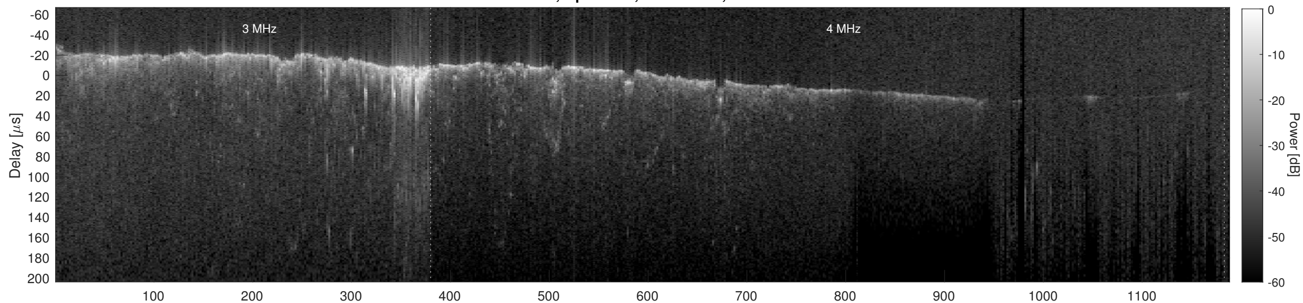
Orbit 8402, Cluttergram
