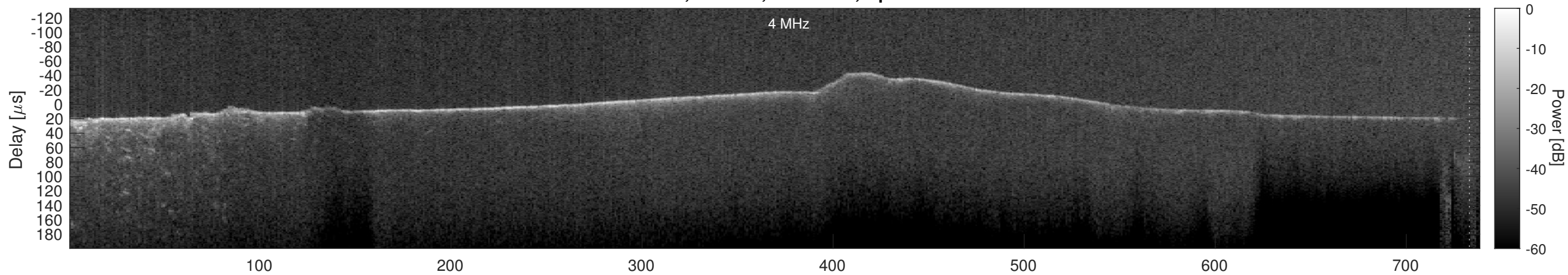
Orbit 8403, Cluttergram
