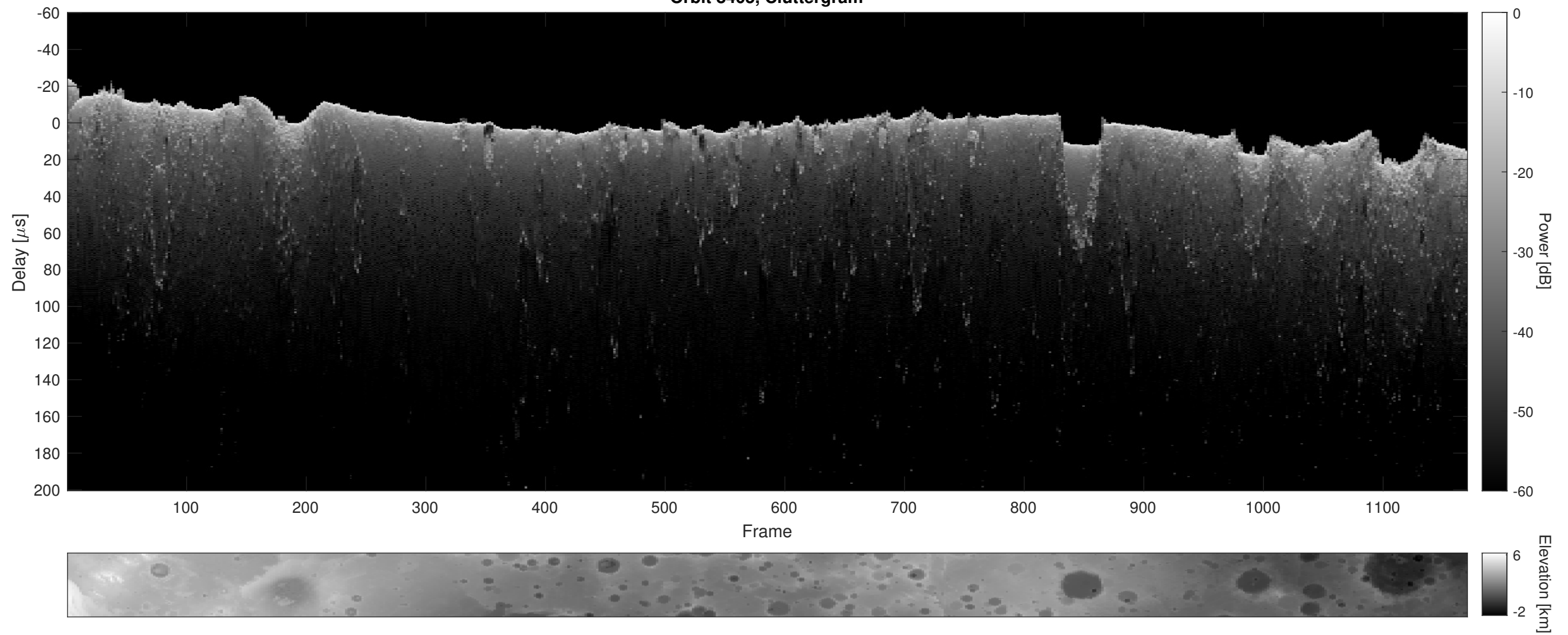
Orbit 8405, Cluttergram
