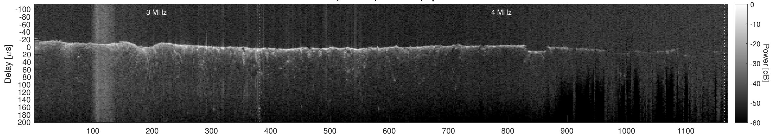
Orbit 8405, Cluttergram
