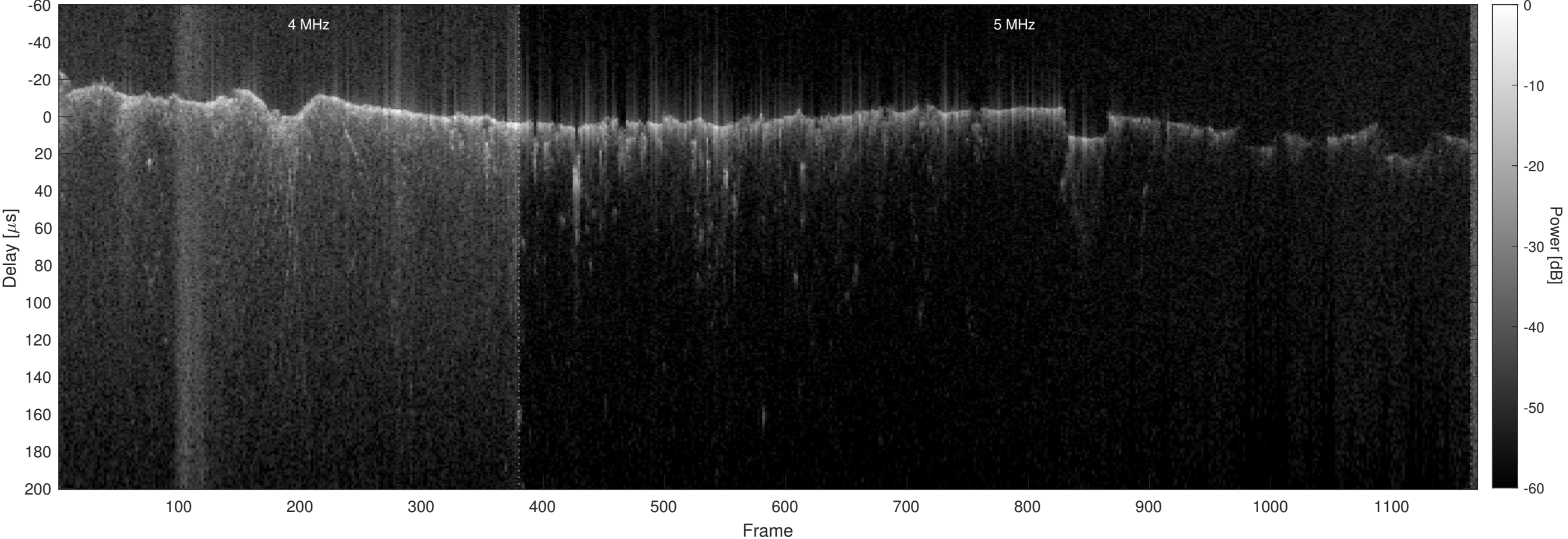
Orbit 8405, Optimized, No Window, Channel 2
