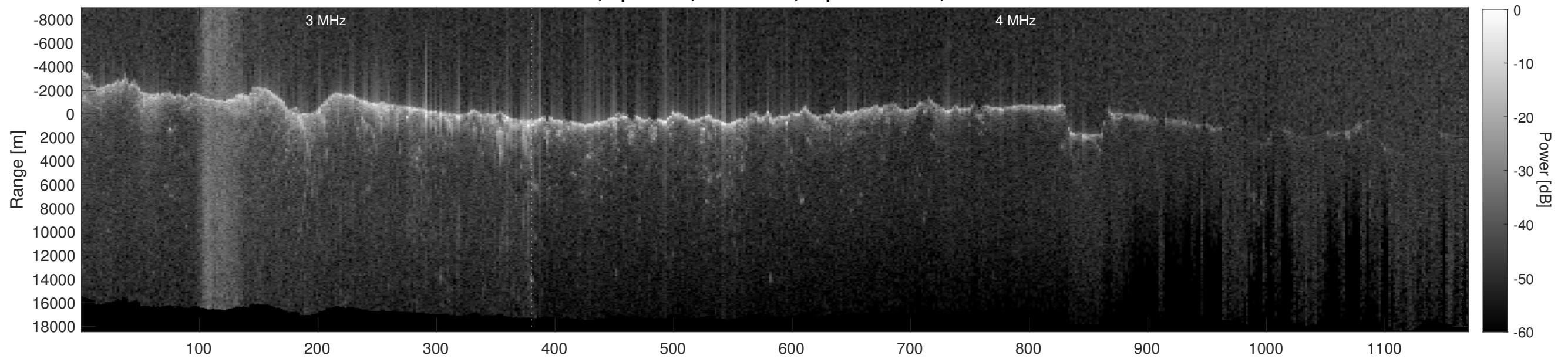
Orbit 8405, Depth-Corrected Cluttergram
