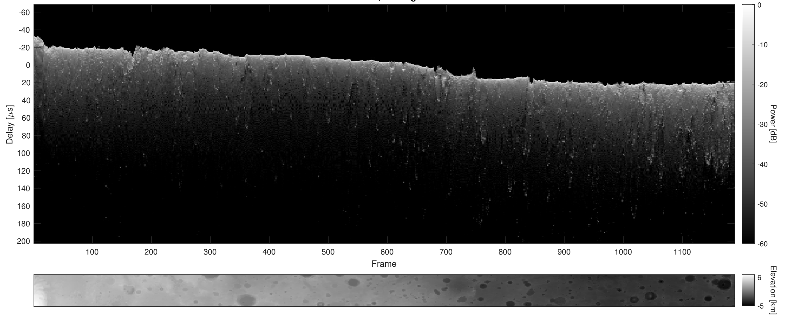
Orbit 8409, Cluttergram
