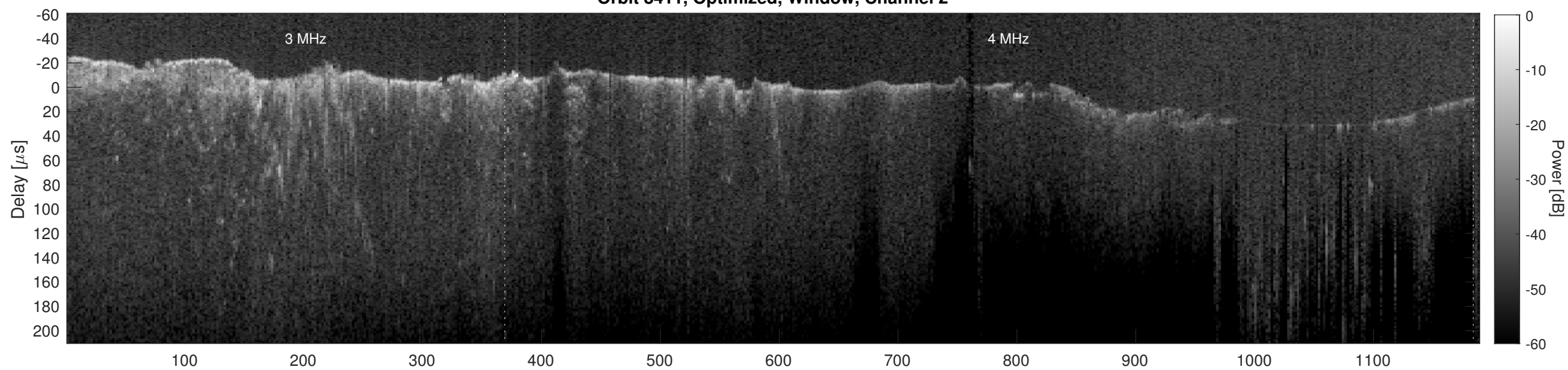
Orbit 8411, Cluttergram
