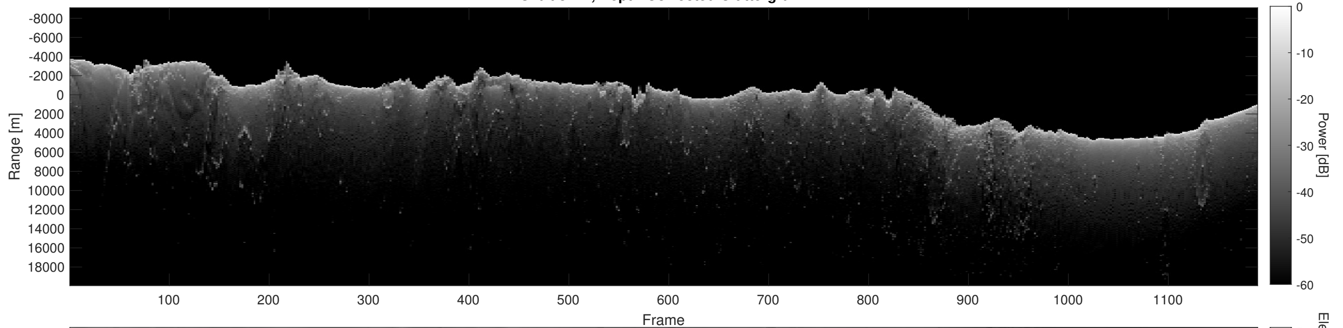
Orbit 8411, Depth-Corrected Cluttergram
