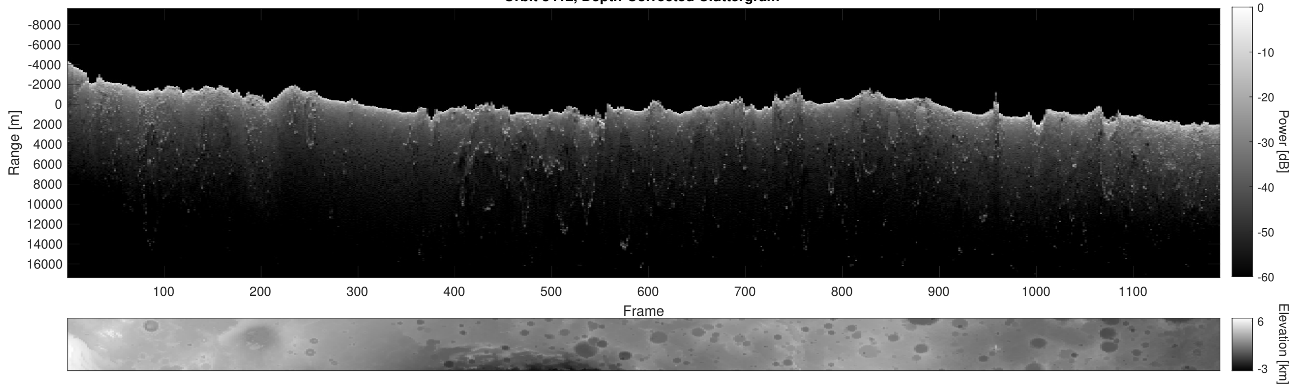
Orbit 8412, Depth-Corrected Cluttergram
