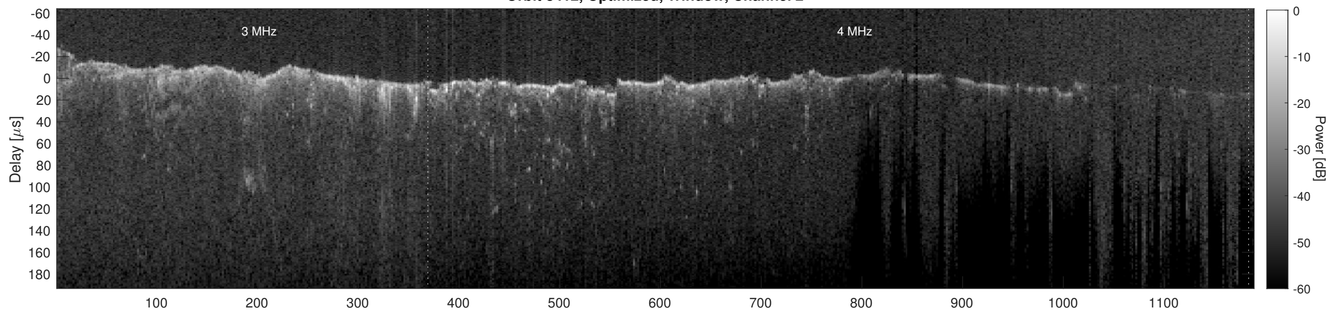
Orbit 8412, Cluttergram
