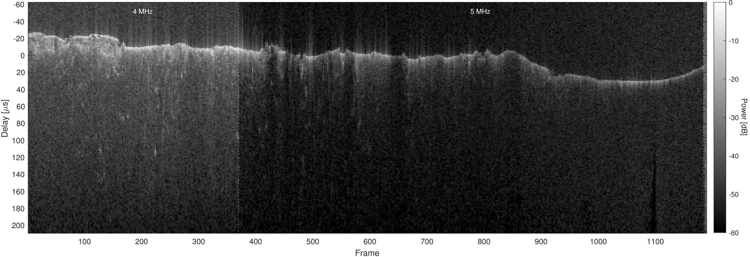
Orbit 8418, Optimized, No Window, Channel 2
