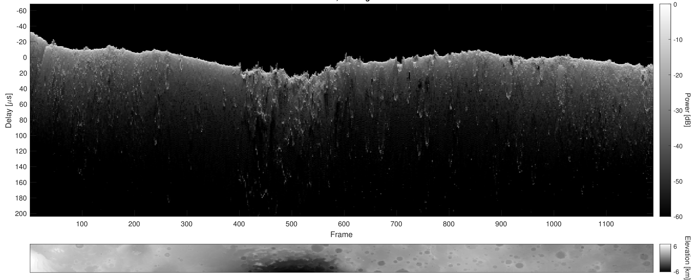
Orbit 8419, Cluttergram
