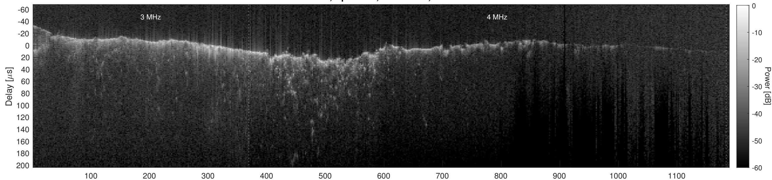
Orbit 8419, Cluttergram
