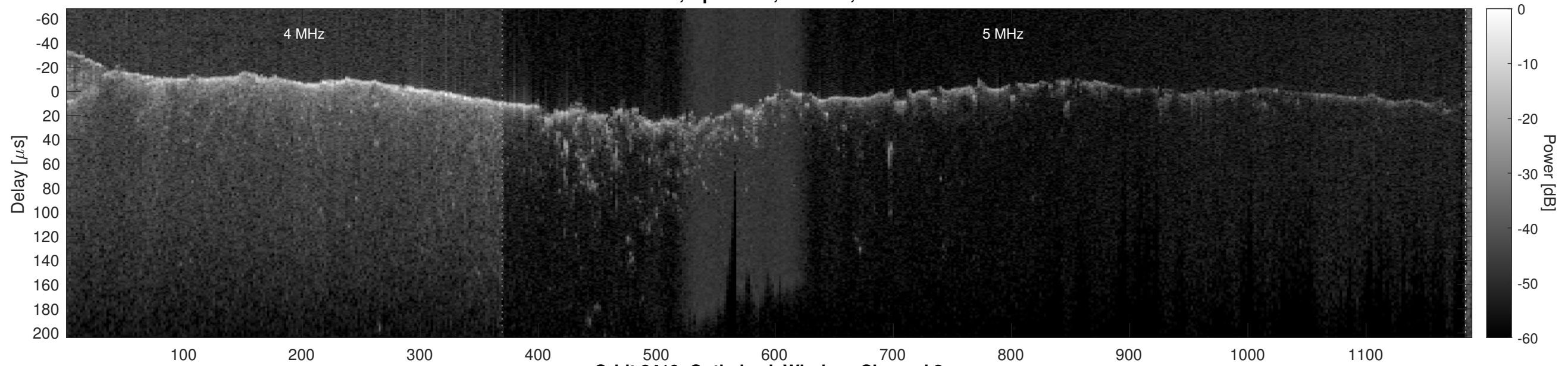
Orbit 8419, Optimized, Window, Channel 2
